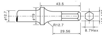
FRH-6A-1 Hexagonal Shank
