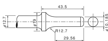
FRH-6A-2 Round Shank
